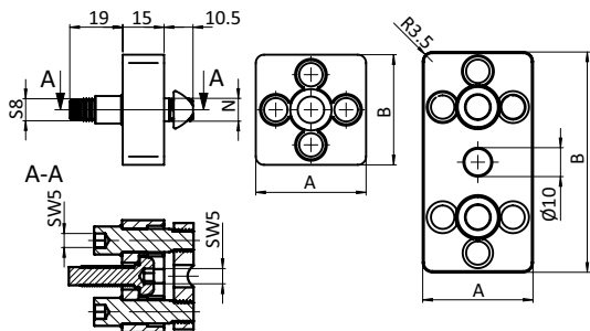
Plate Connector I ZN 40 (Set) Plattenverbinder I ZN 40 (Set)
