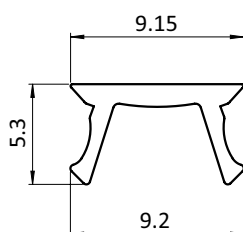
Cover Profile Slot 8 - 4.5 Abdeckprofil Nut 8 - 4,5
