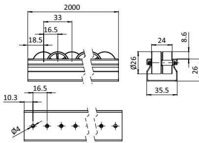
Roller Track XST H26 Rollenschiene XST H26
