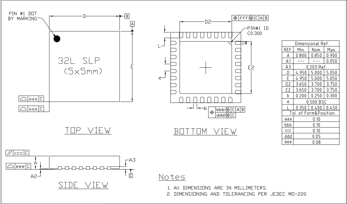
Figure 6-1. ESP8285 Package
