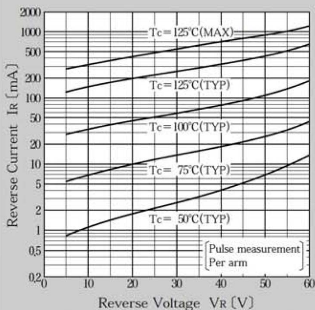
Reverse Current
