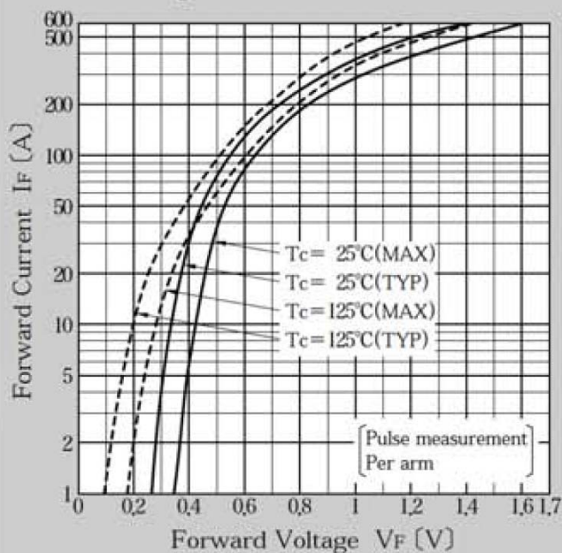
Forward Voltage
