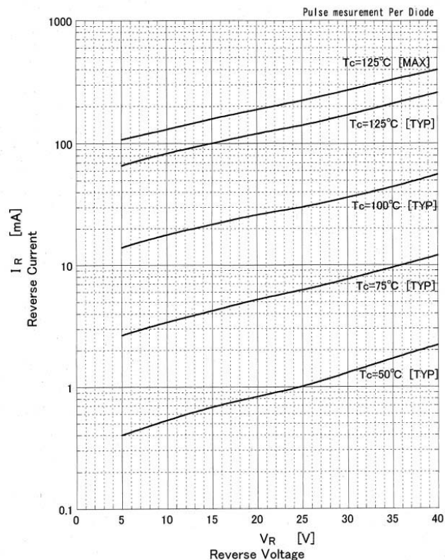
D180SC4M Reverse Current
