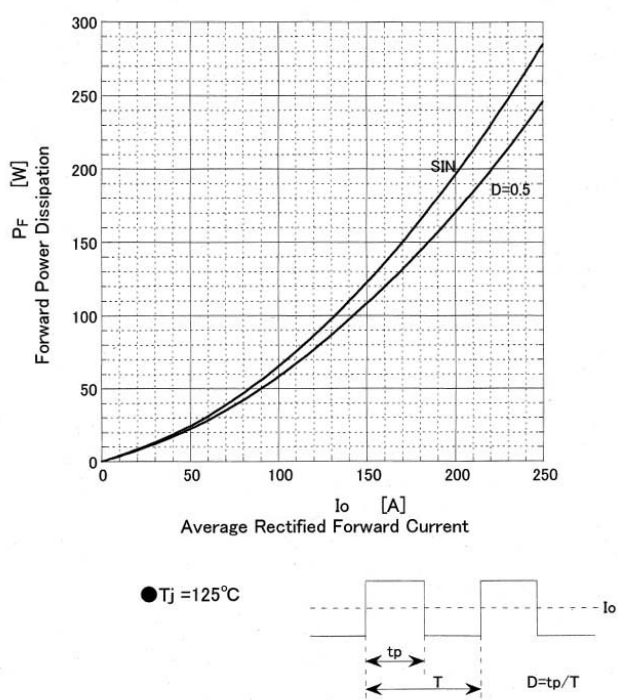
D180SC4M Forward Power Dissipation
