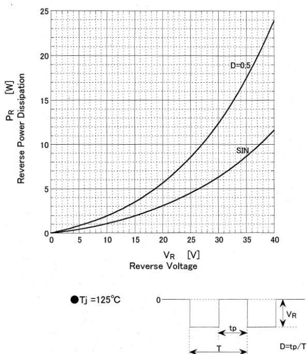
D180SC4M Reverse Power Dissipation
