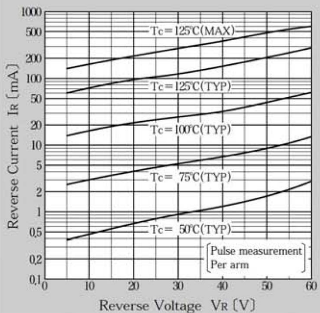
Reverse Current
