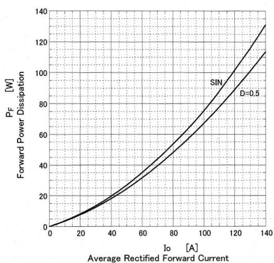
D120SC4M Forward Power Dissipation
