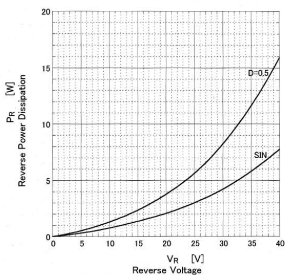
D120SC4M Reverse Power Dissipation
