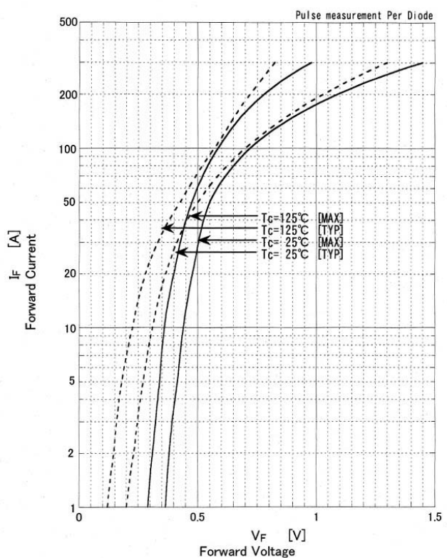
D120SC4M Forward Voltage
