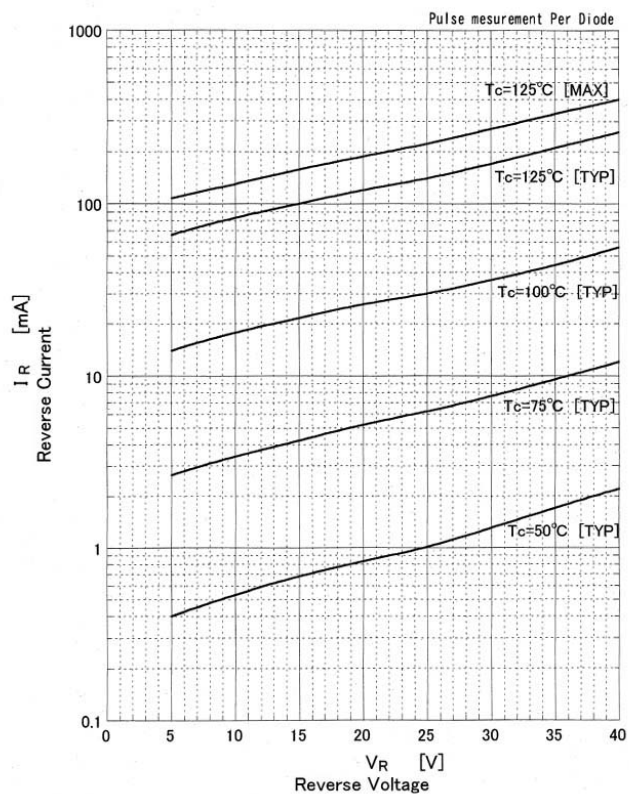
D120SC4M Reverse Current
