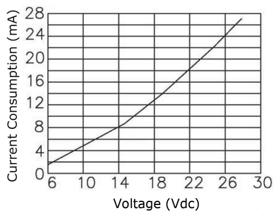
Voltage vs. Current Consumption
