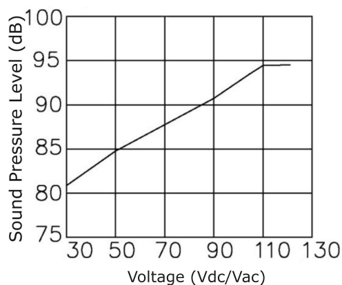
Voltage vs. Sound Pressure Level at 60 cm
