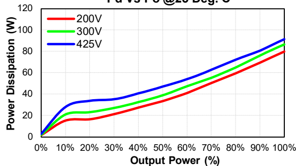
CFB750-300S15 Pd Vs Po @25 Deg. C
