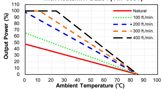
CFB750-300S48 Derating Curve with Heatsink FBL254 (Vin=300V)
