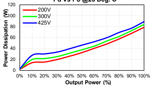
CFB750-300S12 Pd Vs Po @25 Deg. C
