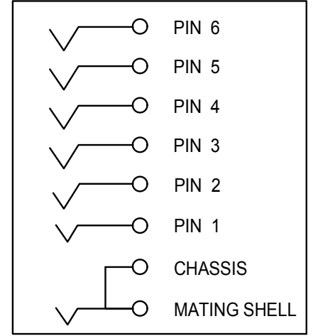
SCHEMATIC CHART
