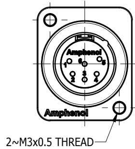
M3 THREAD OPTION
