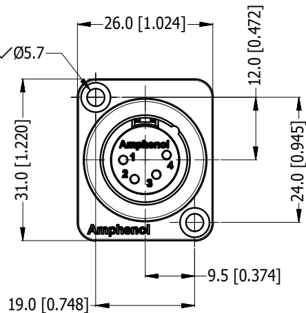
THROUGH HOLE
