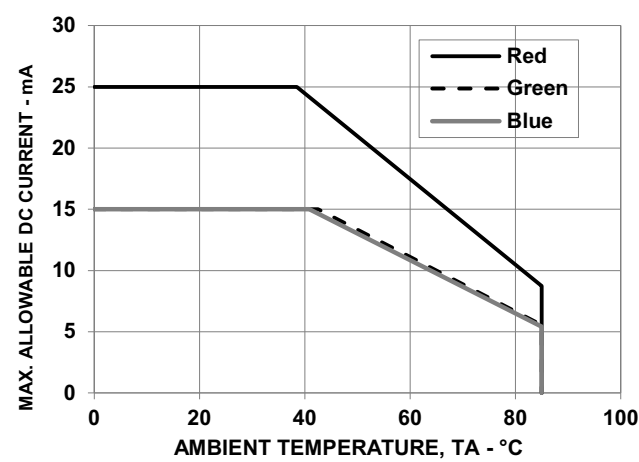
Figure 8: Maximum Forward Current vs. Temperature for Red, Green, and Blue
