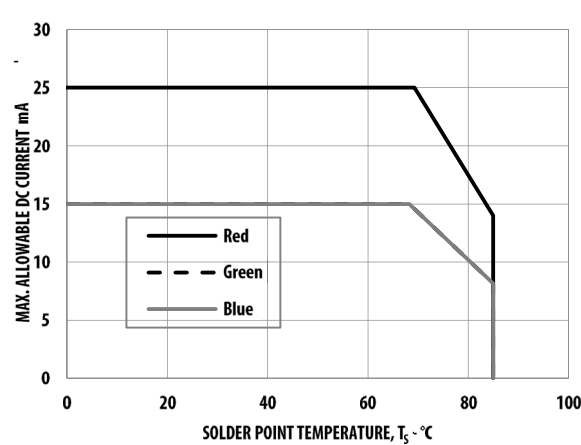
Figure 9: Maximum Forward Current vs. Solder Temperature for Red, Green, and Blue
