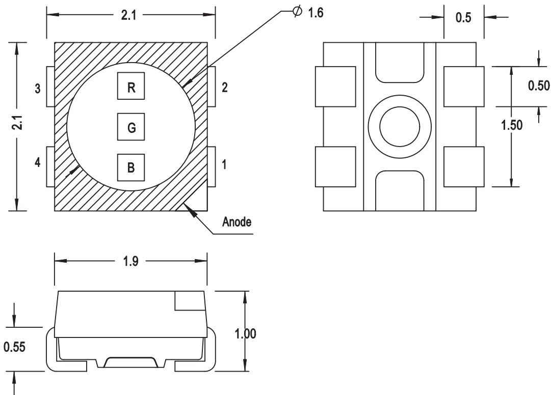
Figure 1: Package Drawing
