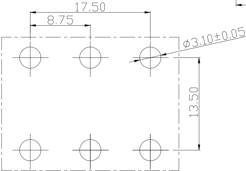
PCB LAYOUT
