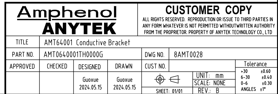
Technical Specification: 1. Material: Copper alloy ,Matte Tin Plated 2. Current: 135A. 3. Torque: 15 lbf.in. 4.Mark "▲" is the Critical dimension.
