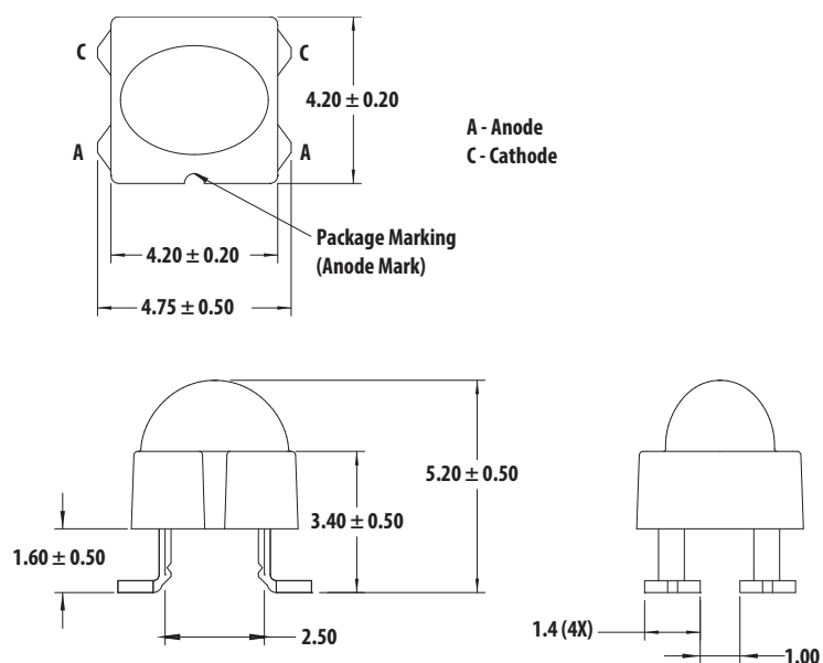
Figure 1: Package Dimensions
