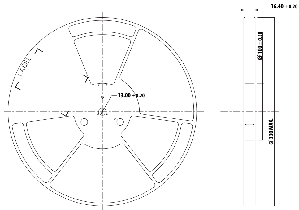
Figure 18: Reel Dimensions
