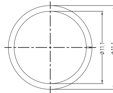
SPRING WASHER
