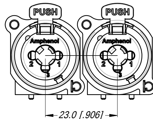
MIN MOUNTING PITCH
