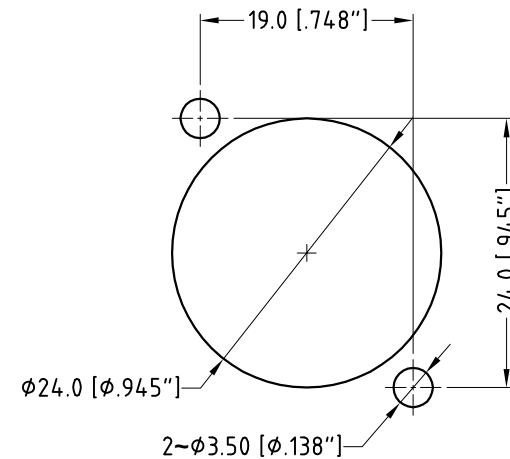
PANEL CUTOUT
