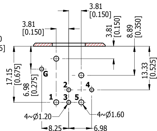
PCB LAYOUT COMPONENT SIDE TOLERANCE: \pm 0.05\text{mm} [.002"]
