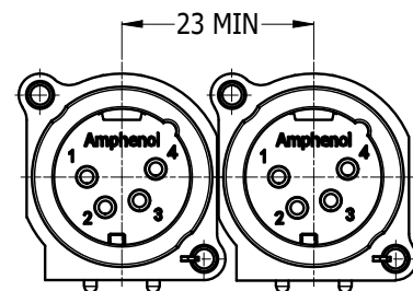
MINIMUM MOUNTING PITCH (SCALE 1 : 1)
