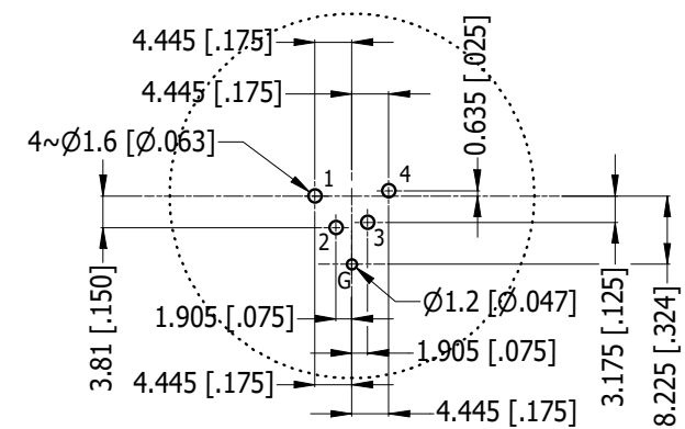
PCB LAYOUT CONNECTOR SIDE
