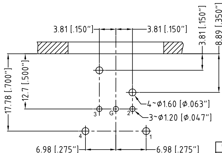
PCB-LAYOUT COMPONENT SIDE TOLERANCE:±0.05mm[.002"]
