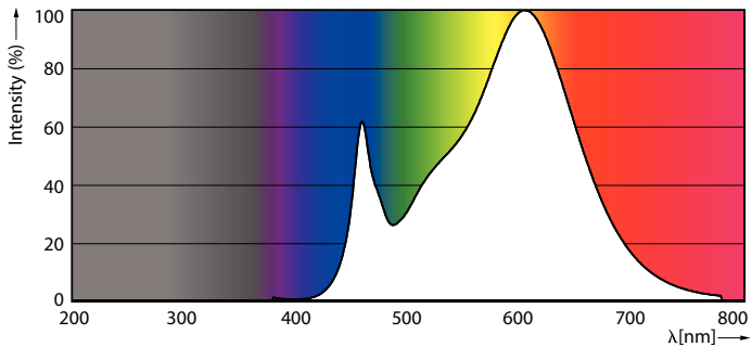
LEDcapsule LV 1,8W GY6,35 830
