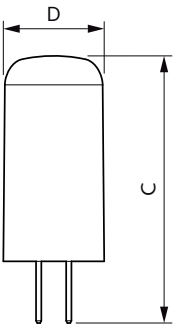
GY6.35 1.9W-20W 200lm 3000K Non-Dim
