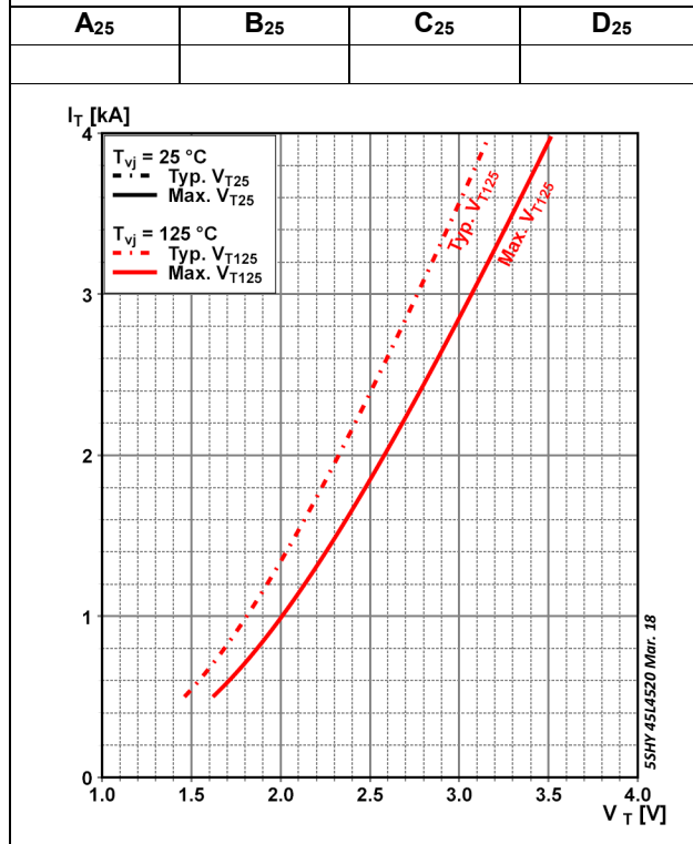
Fig. 3 GCT on-state voltage characteristics
