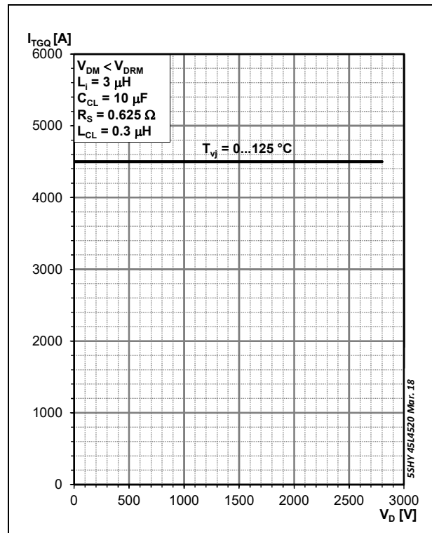
Fig. 8 Safe Operating Area
