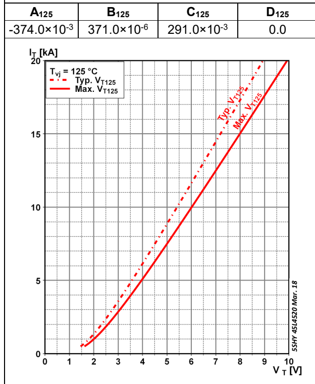
Fig. 4 GCT on-state voltage characteristics
