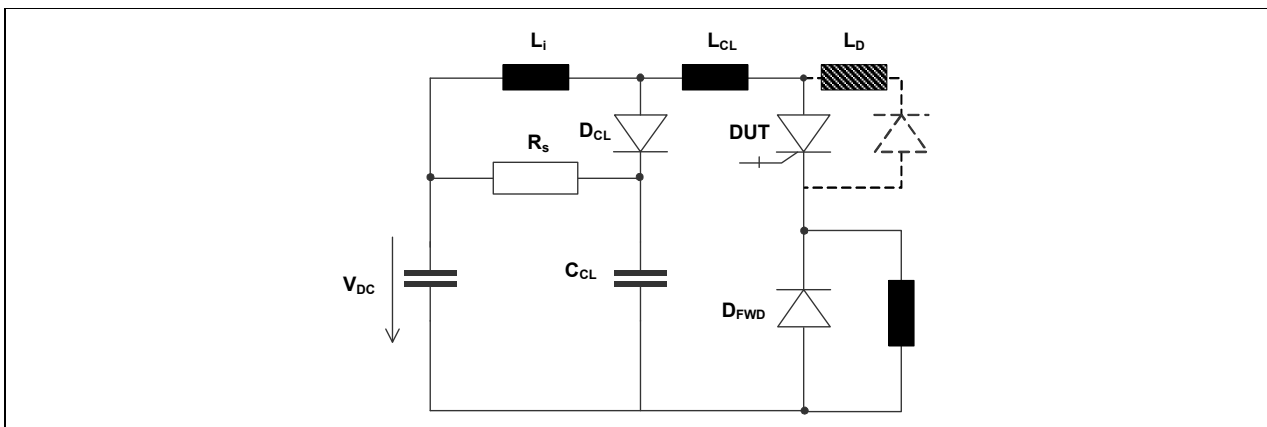
Fig. 15 Test circuit
