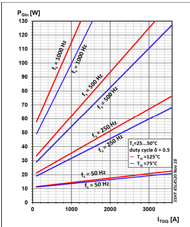
Fig. 9 Max. Gate Unit input power in chopper mode
