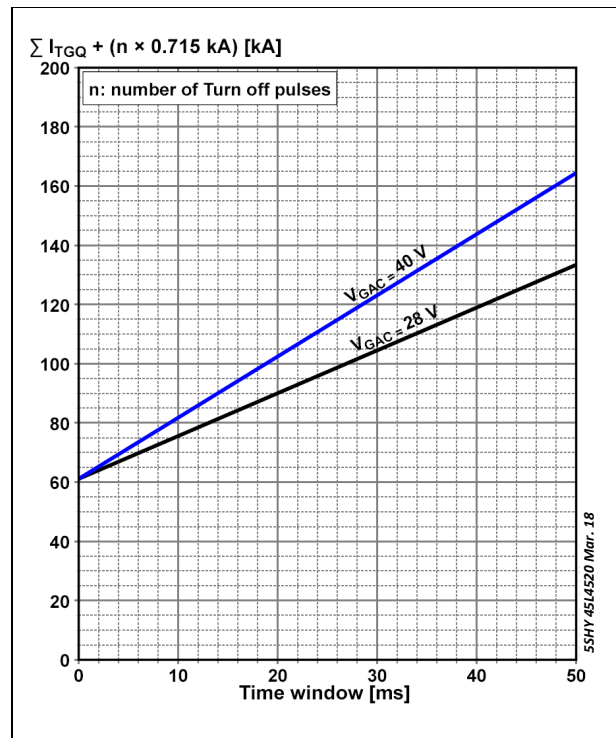
Fig. 10 Burst capability of Gate Unit
