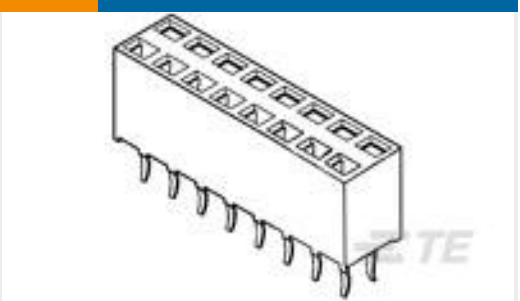
TE Model / Part #2-215307-9 2X29P HV100 REC CON. TE, 7.0MM
