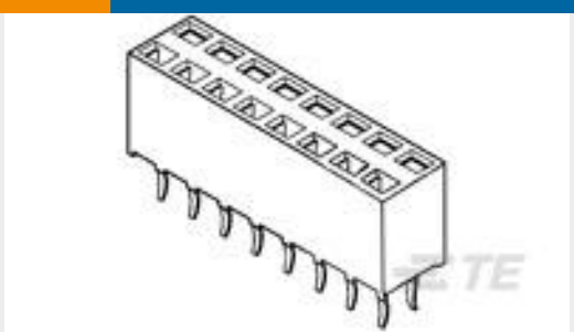
TE Model / Part #3-215307-2 2X32P HV100 REC CON. TE, 7.0MM
