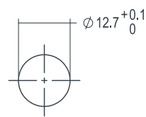
Mounting Hole
