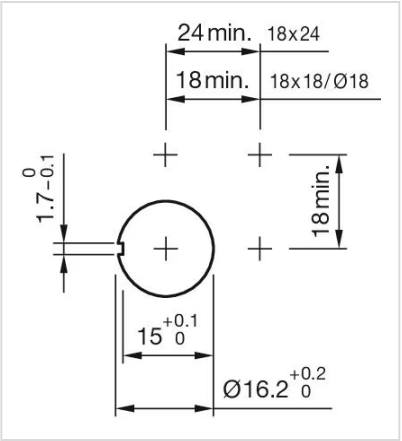
Dimension drawings:
