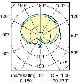
LED Lamps, LEDClassic 60W A60 E27 2700K 806lm FR
