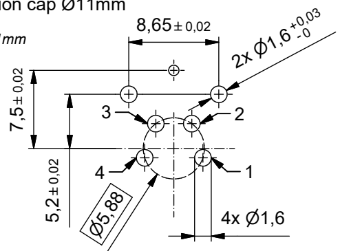
Top view Layout PCB/ Leiterplatte
