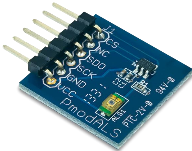
The PmodALS.
