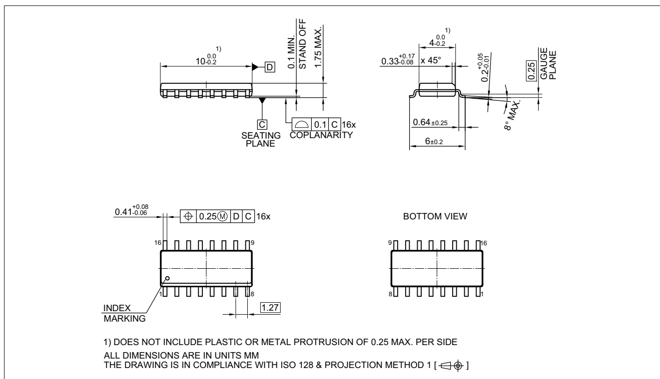
Figure 16 PG-DSO-16-11 outline
