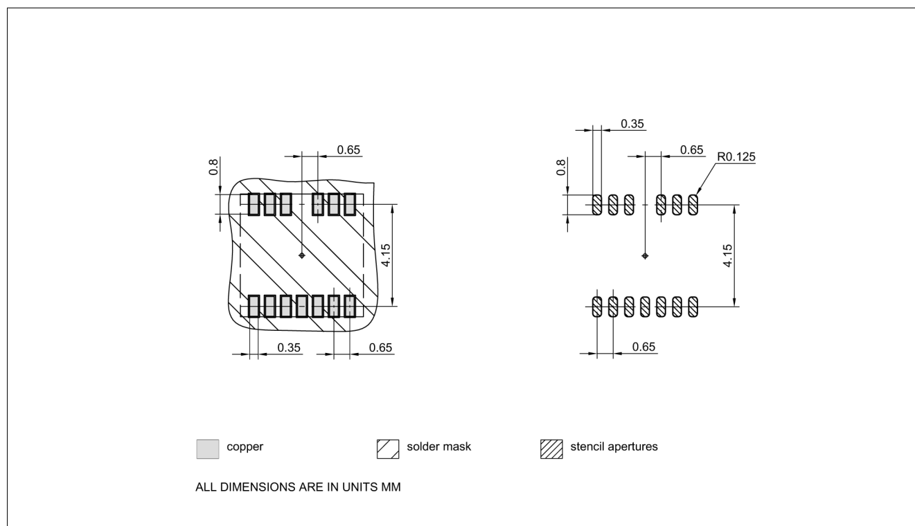
Figure 23 PG-TFLGA-13-1 footprint
