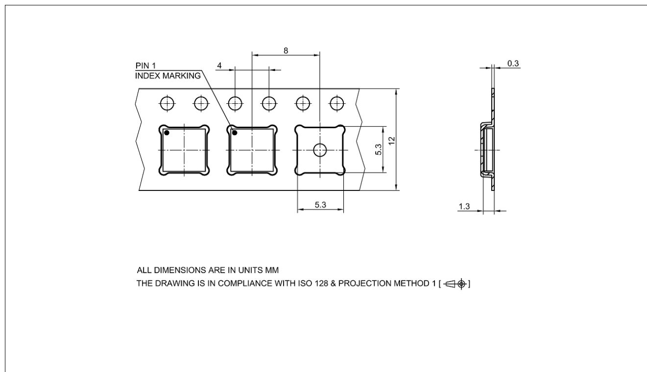
Figure 24 PG-TFLGA-13-1 packaging
