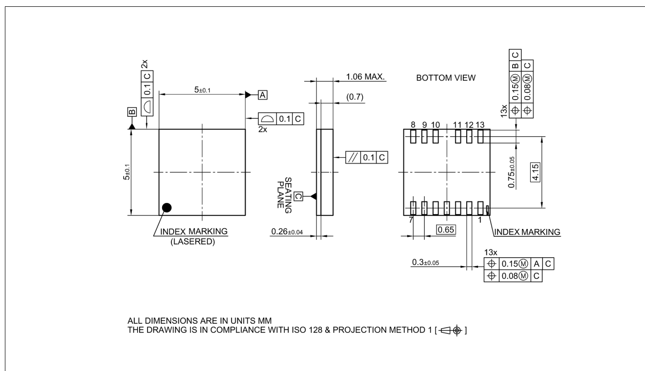
Figure 22 PG-TFLGA-13-1 outline
