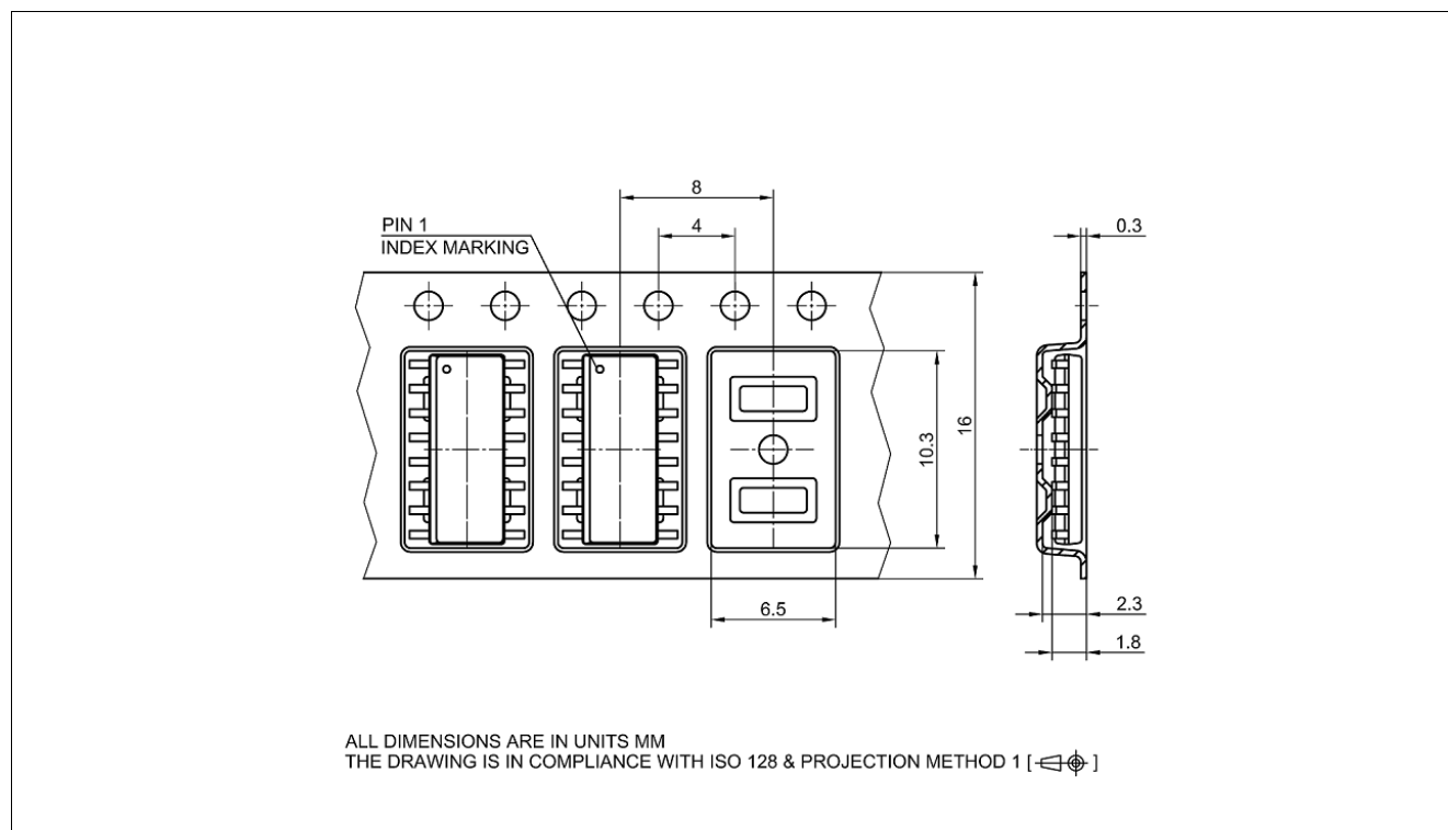
Figure 18 PG-DSO-16-11 packaging
