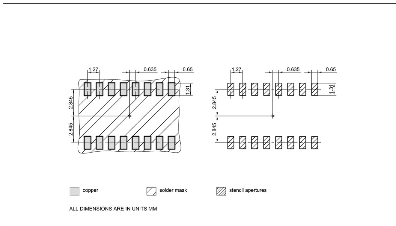
Figure 17 PG-DSO-16-11 footprint
