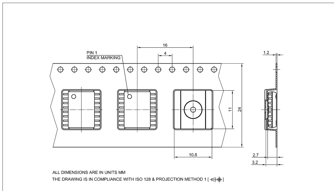
Figure 21 PG-DSO-16-30 packaging
