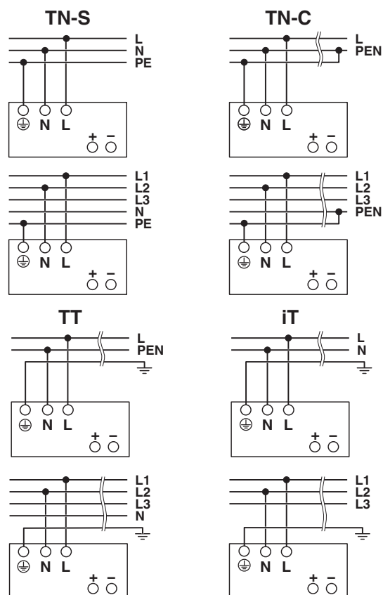
Figure 17 Network types
