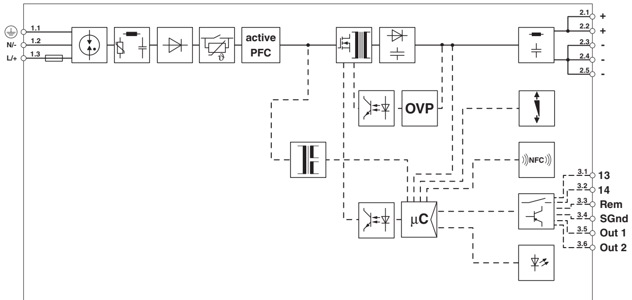
Figure 7 Block diagram
