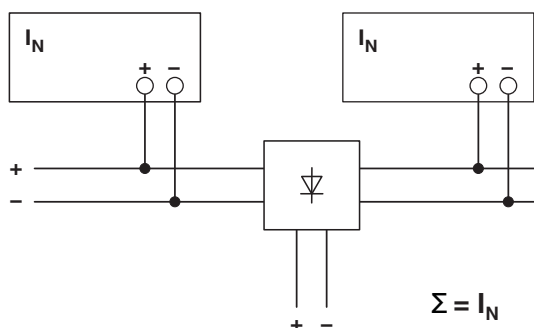
Figure 46 Schematic diagram, redundant operation with QUINT DIODE
