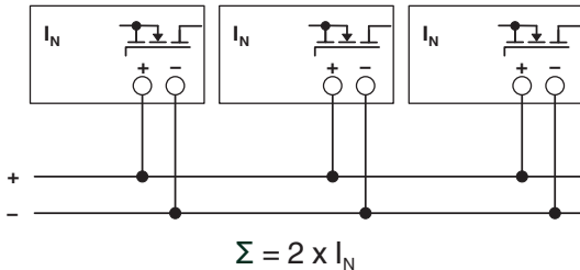
Figure 47 Schematic diagram, n+1 redundant operation for 40 A output current
