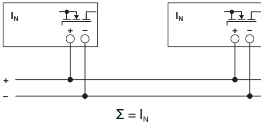
Figure 46 Schematic diagram, 1+1 redundant operation for 20 A output current
