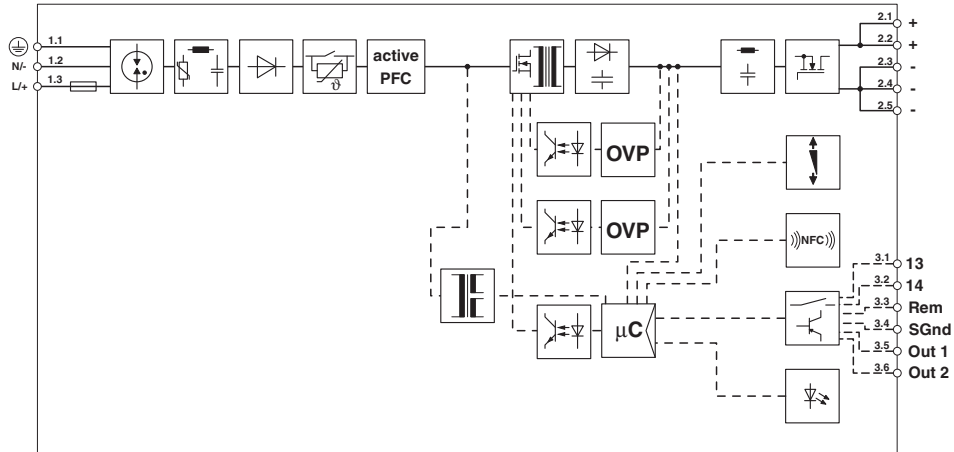
Figure 7 Block diagram
