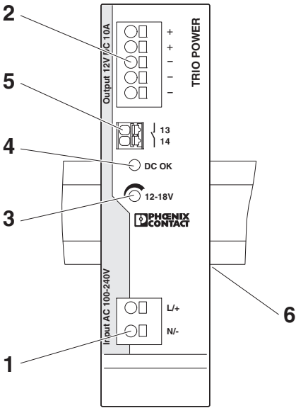
Figure 3 Function elements
