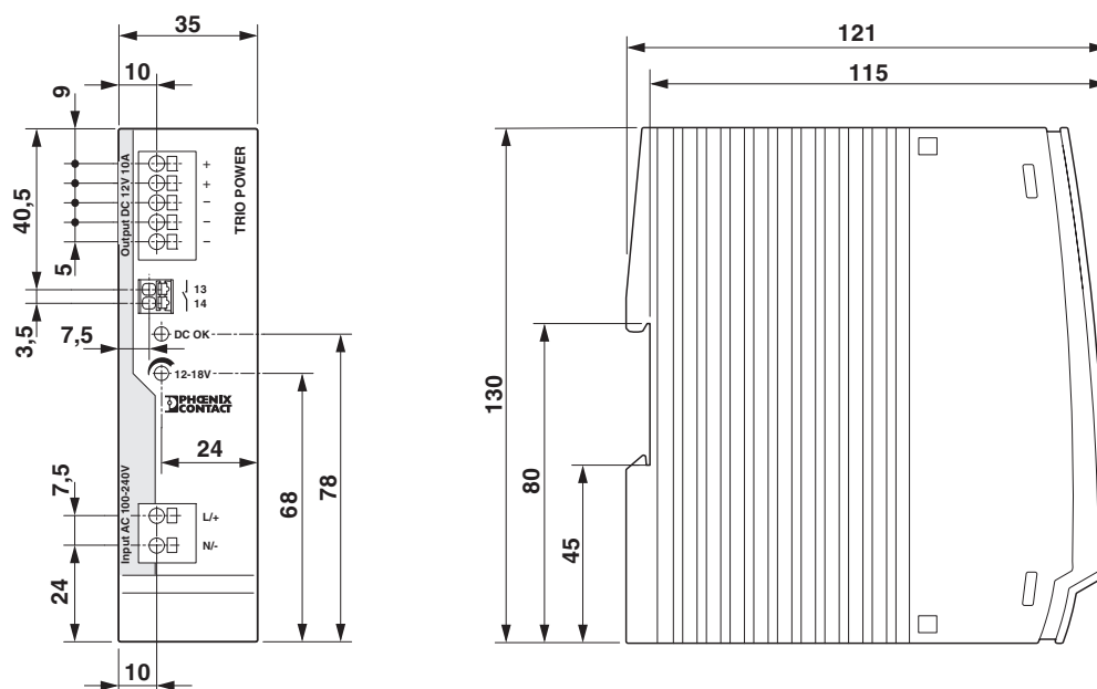
Figure 6 Device dimensions
