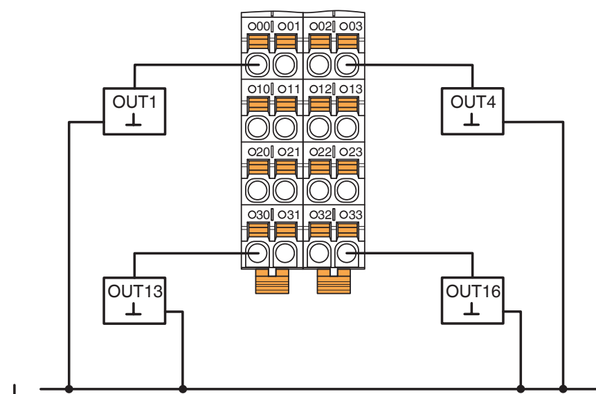
Connection diagram
