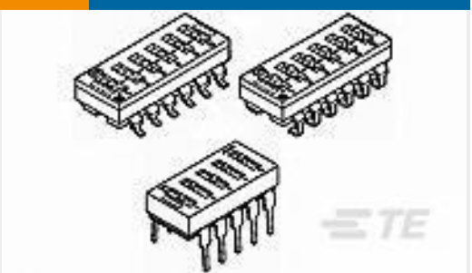
TE Model / Part #1825360-4 ADE06A04=6 POS DIP SWITCH
