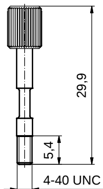
JACK SCREW (1x)
