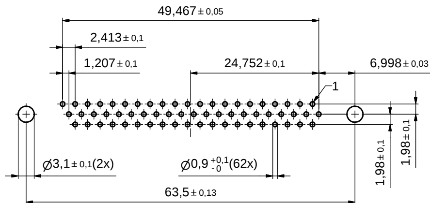
P.C.B. HOLE DRILLINGS
