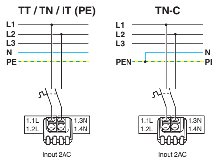
Figure 16 Schematic diagram, two-phase fuse protection
