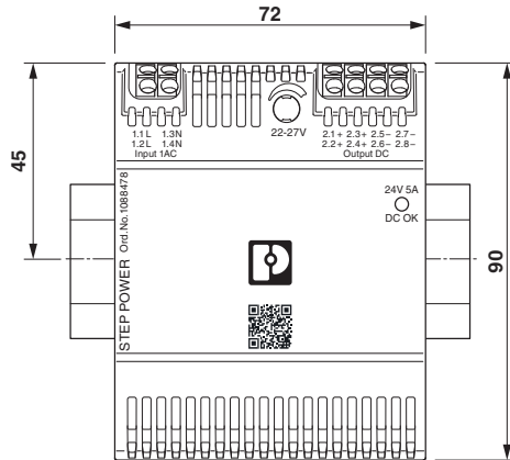
Figure 5 Device dimensions (dimensions in mm)
