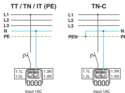
Figure 15 Schematic diagram, single-phase fuse protection
