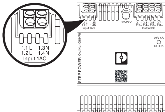
Figure 14 Position of the AC input terminal blocks
