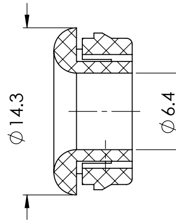
SECTION Y-Y
