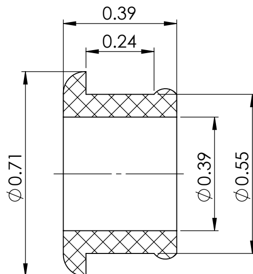
SECTION Y-Y
