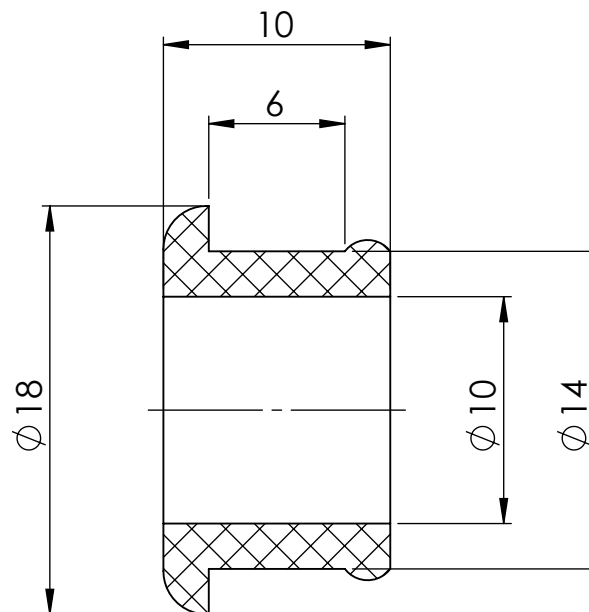
SECTION Y-Y
