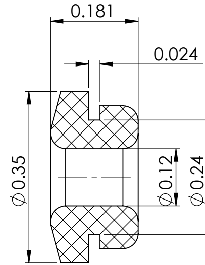
SECTION Y-Y
