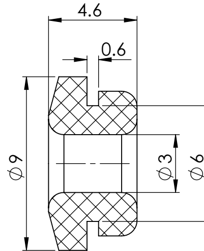
SECTION Y-Y
