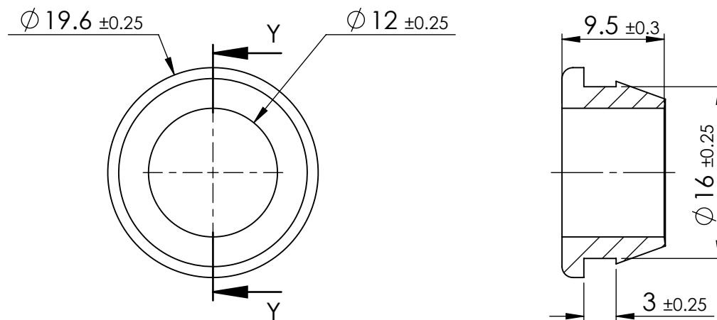
SECTION Y-Y
