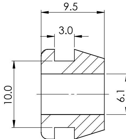
SECTION Y-Y
