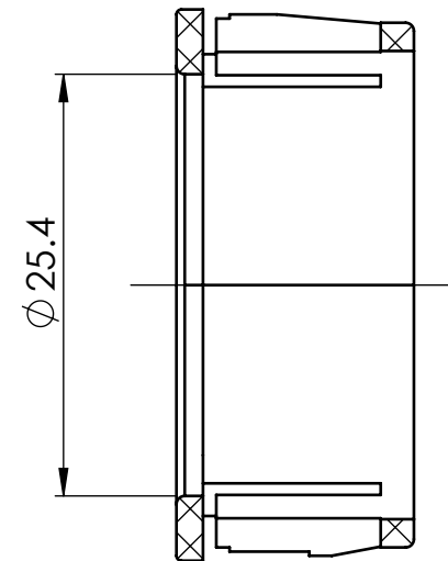
SECTION Y-Y
