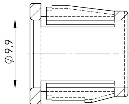
SECTION Y-Y
