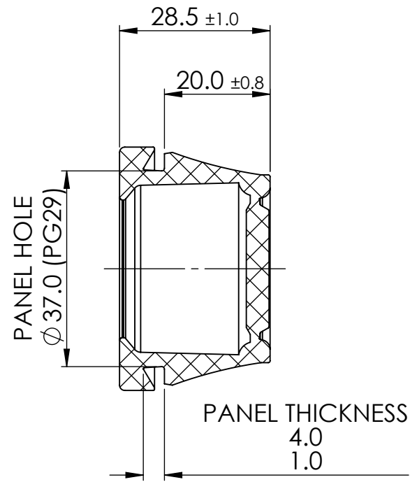
SECTION Y-Y
