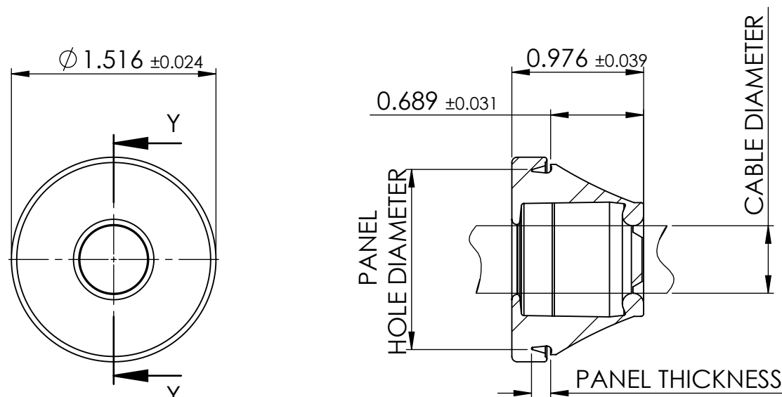
SECTION Y-Y
