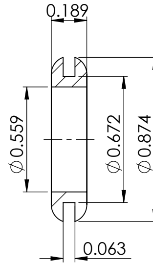
SECTION Y-Y
