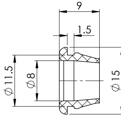
SECTION Y-Y
