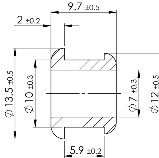
SECTION Y-Y
